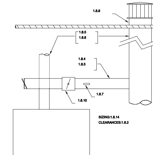
FIG. 1.8.1: VENT DESIGN INSTRUCTION - REFERENCES
