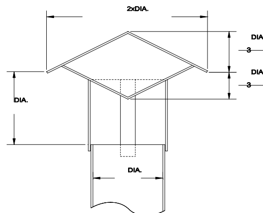
FIG. 1.8.9B: LOW RESISTANCE VENT CAP
