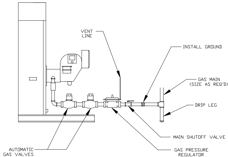
FIGURE 1.5A: GAS BURNER CONNECTION
