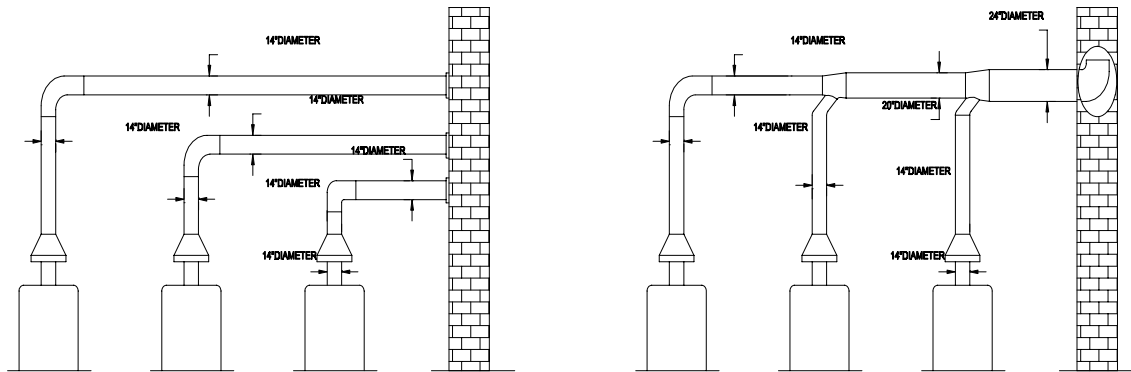
FIG. 1.8.11: SUGGESTED APPLIANCE VENTING PROCEDURE
