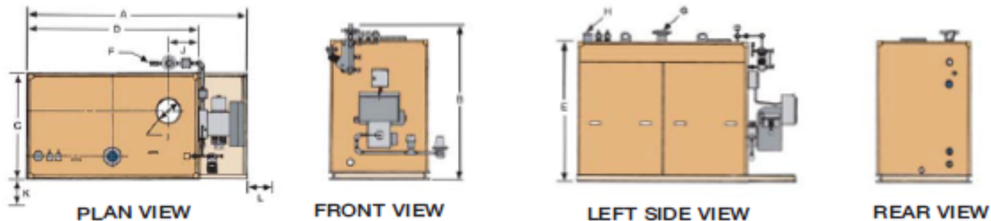
STEAM BOILER DIMENSIONS in inches (cm)
