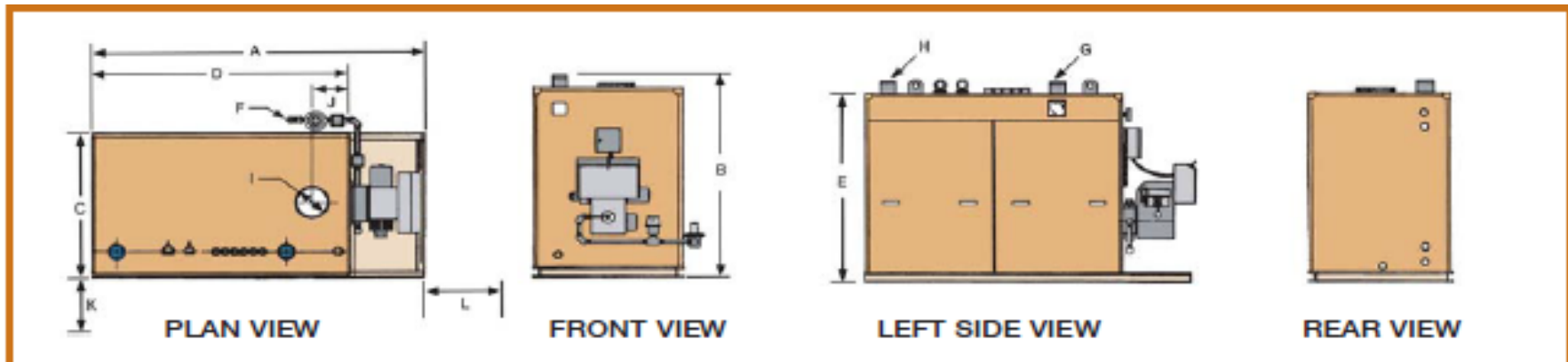
WATER BOILER DIMENSIONS in inches (cm)
